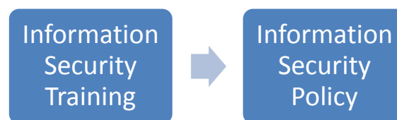
Figure 1.1: Fundamental Argument
