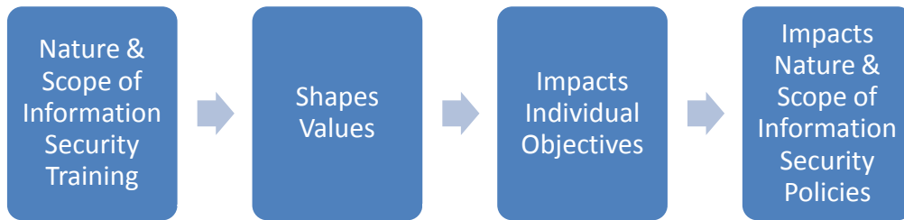
Figure 1.2: Detailed Argument
